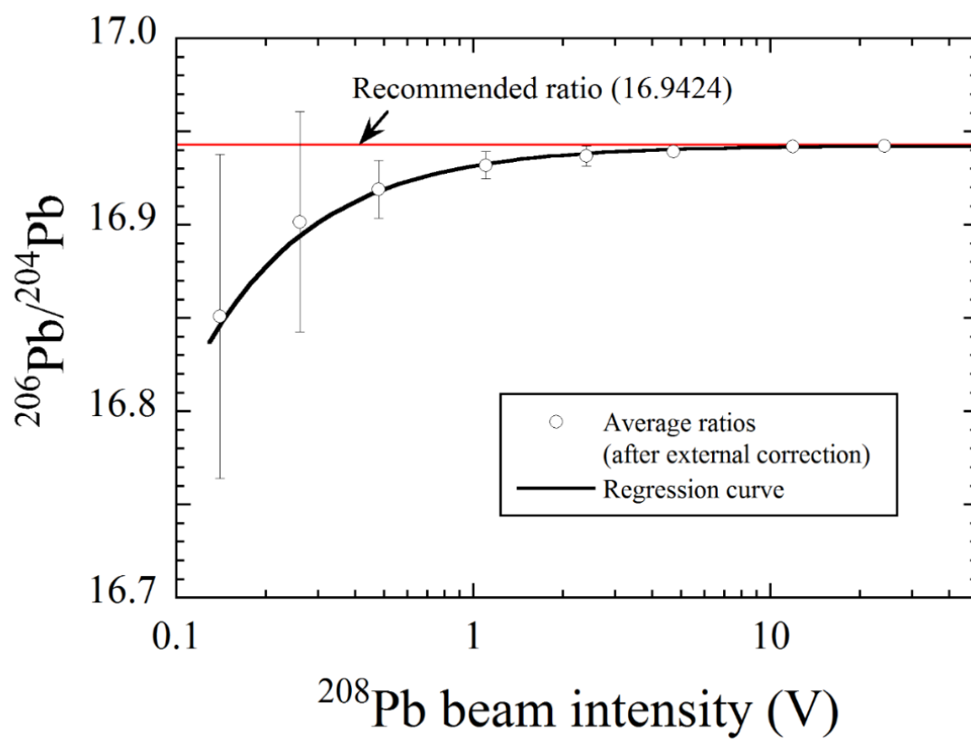
Fig. 2. The results of replicate analyses on NIST981 for variable sample sizes, showing the average ^{206}\text{Pb}/^{204}\text{Pb} ratios with error bars ( 2\sigma ) as a function of the ^{208}\text{Pb} beam intensity (V).
