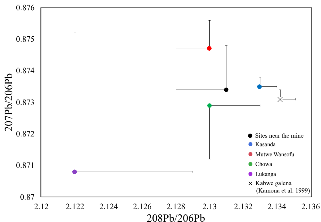
Fig. 5. Pb isotope ratios ( ^{208}\text{Pb}/^{206}\text{Pb} and ^{207}\text{Pb}/^{206}\text{Pb} ) in the blood of the dogs residing in different areas ( n = 119 ). The mean values are shown with error bars indicating the SD.
